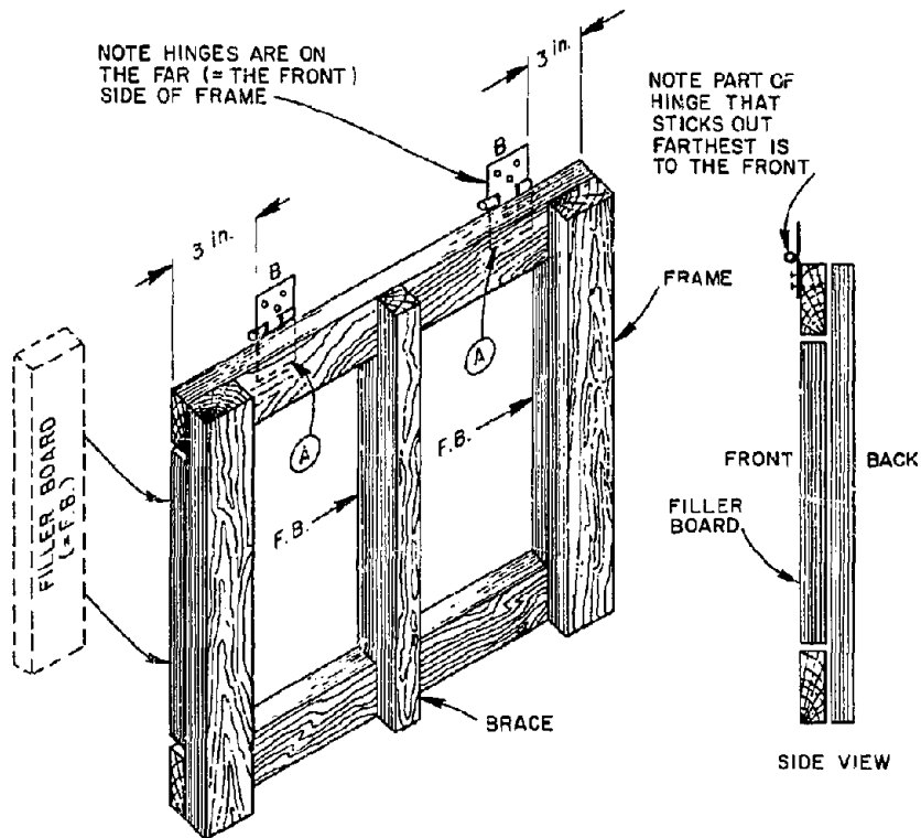
Fig. B-4. Completing the frame.
